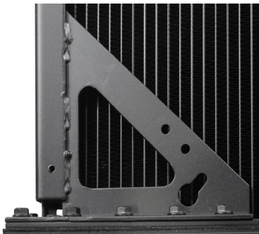
Welded Construction and Powder-Coat Finish on Side Frame and Tanks
