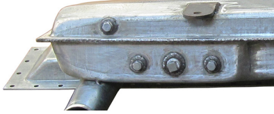
Zinc Coated Steel Header and Expansion Tanks for Extended Corrosion Protection
